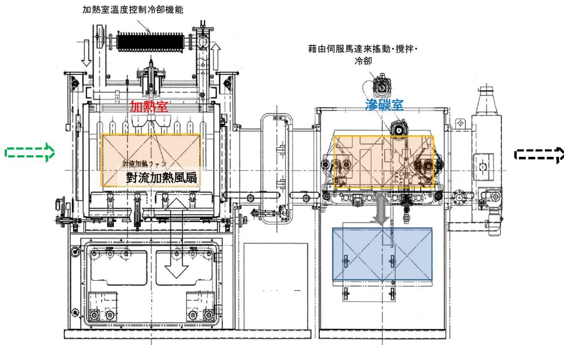
E-TKM80直通式真空滲碳爐
